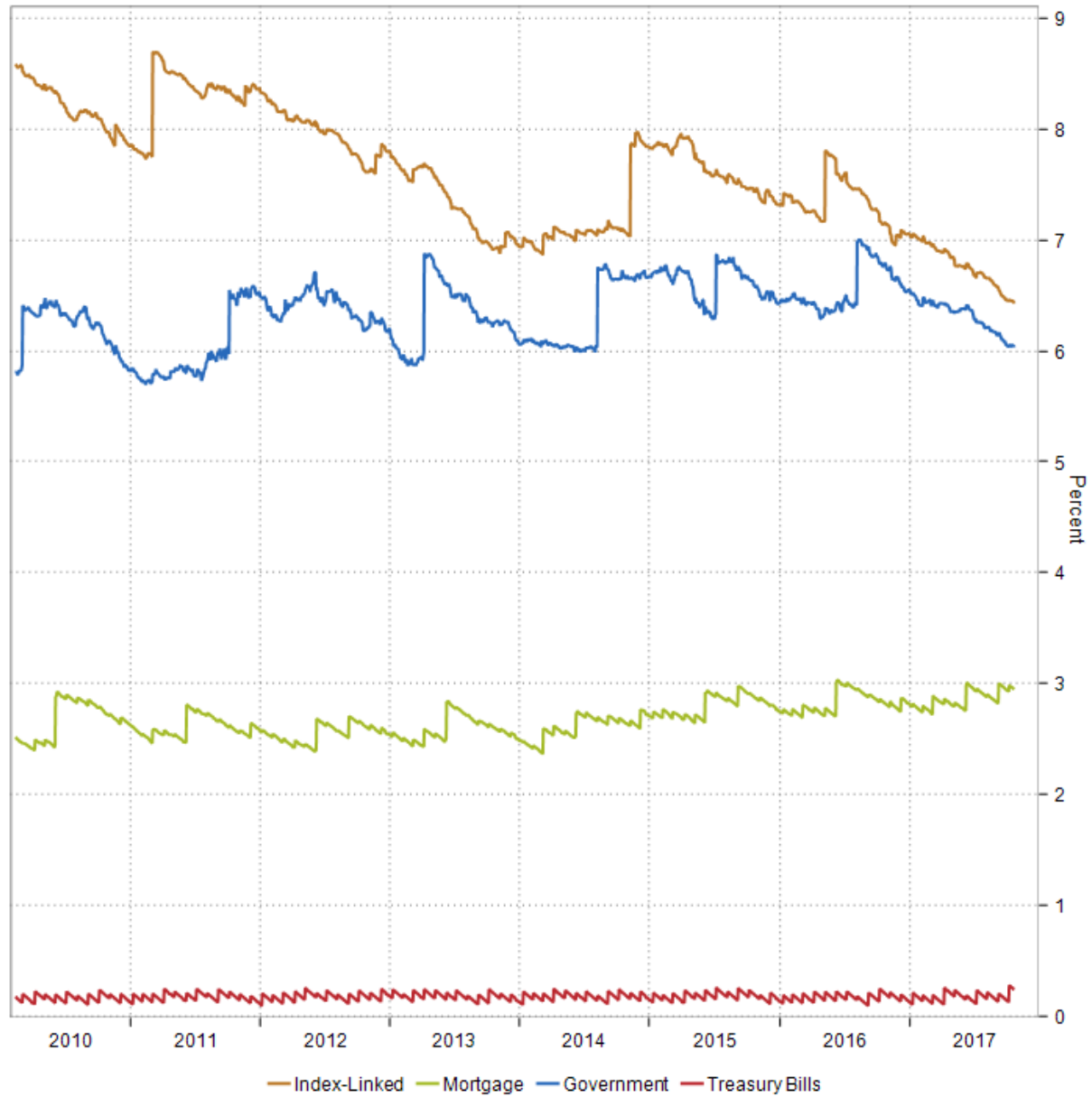
Swedish Fixed Income - Modified Duration
